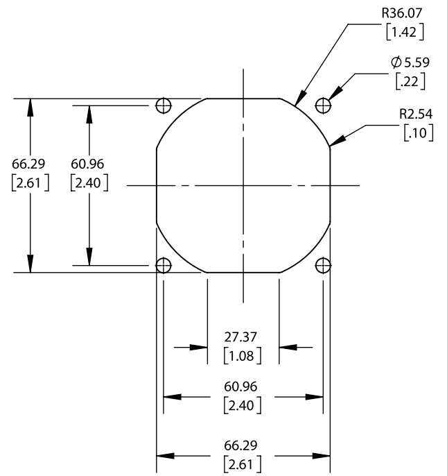
MOUNTING CUTOUT DIMENSIONS
